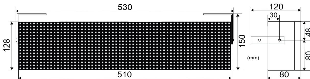
Fig. 2 DISBRSE dimensions
